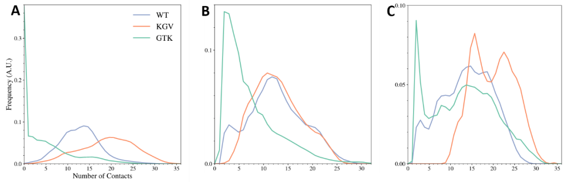
Figure 10. Inter-domain contacts in WT, KGV, and GTK a-syn variants. The distribution of inter-domain contacts between the N-terminal and C-terminal domains ( a ), the NAC and C-terminal domains ( b ), and the N-terminal and NAC domains ( c ) shows that the GTK mutations leads to significantly reduced interactions between the C-terminal domain and the other two domains. The contact distributions also show that that the KGV mutations leads to a large increase in the number of contacts between the N-terminal and NAC domains.
