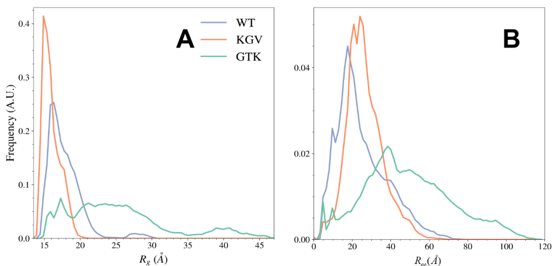
Figure 9. Radius of gyration and end-to-end distance measurements for WT, KGV, and GTK a-syn variants. Comparison of the radius of gyration, R_g (a), and the end-to-end distance, R_{ee} (b) for the WT, KGV, and GTK protein variants shows that the GTK mutant can sample much more elongated structures than either the WT or KGV variants, due to the decrease in interactions between the C-domain and the rest of the protein. The KGV mutant, on the other hand, samples structures that are more compact, due to increased contacts between the N-terminal and NAC domain and increased sampling of beta sheet rich structures.
